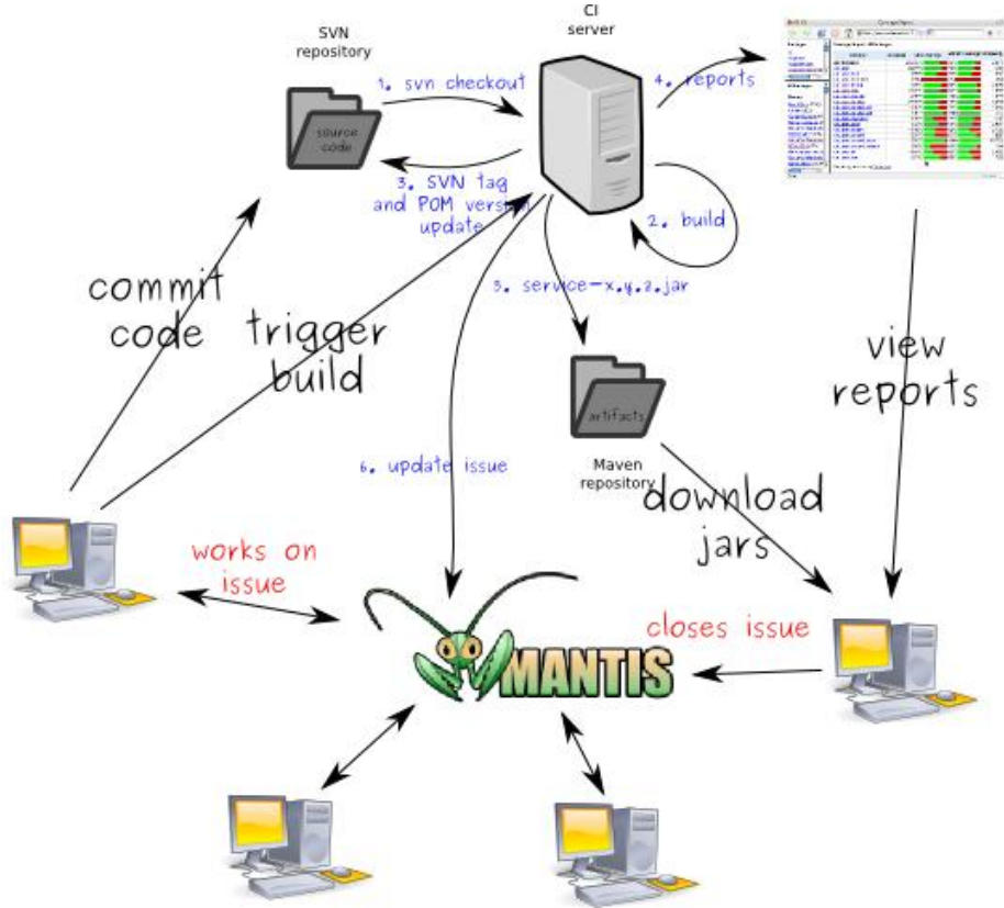
10: Development infrastructure
